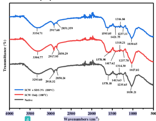
Figure 6. FTIR spectrum on the native, SCW-treated, and SCW+SDS-treated substrates (180 °C, 60 bar, 60 min).
